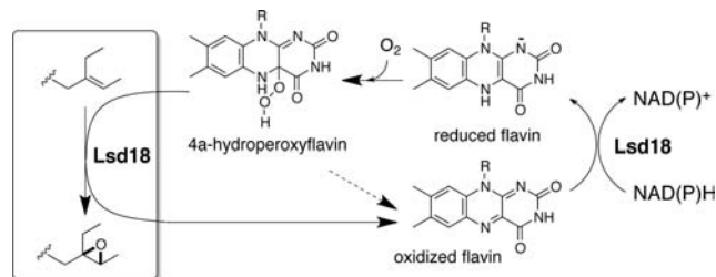
Figure 4. Reaction mechanism of Lsd18 catalyzed epoxidation.
